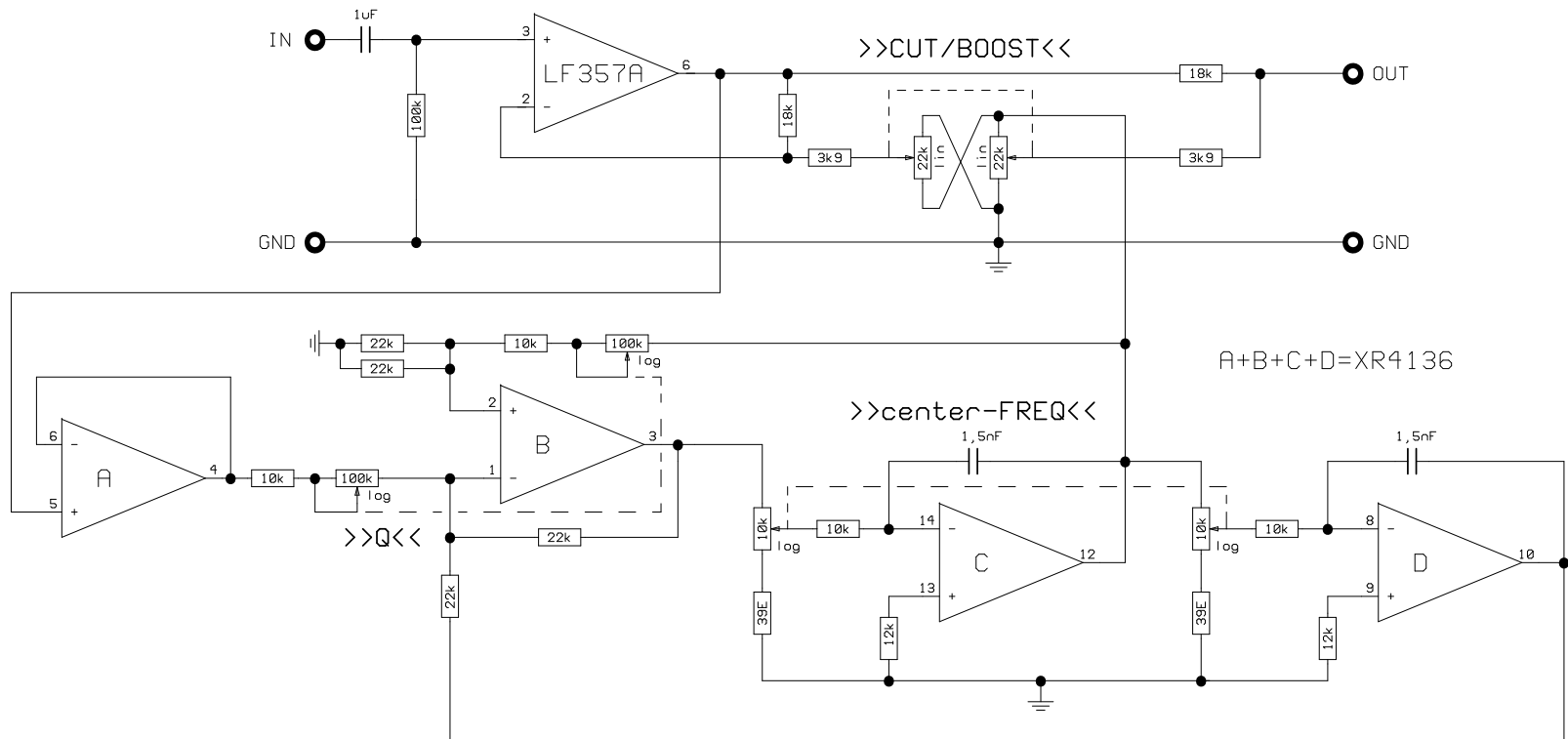
Parametric Equaliser Filter section
